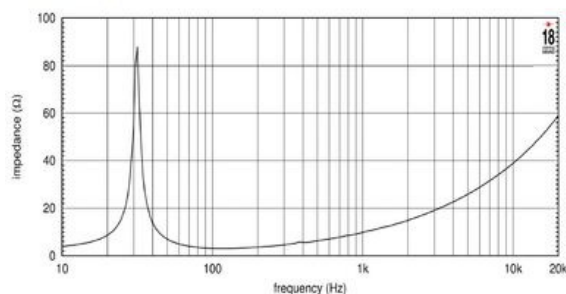
FREE AIR IMPEDANCE CURVE
