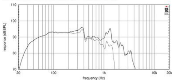
FREQUENCY RESPONSE MADE IN 180 LT. ENCLOSURE TUNED AT 35 Hz IN FREE FIELD (4π) ENVIRONMENT. ENCLOSURE CLOSES THE REAR OF THE DRIVER, THE THIN LINE REPRESENTS 45° OFF AXIS FREQUENCY RESPONSE
